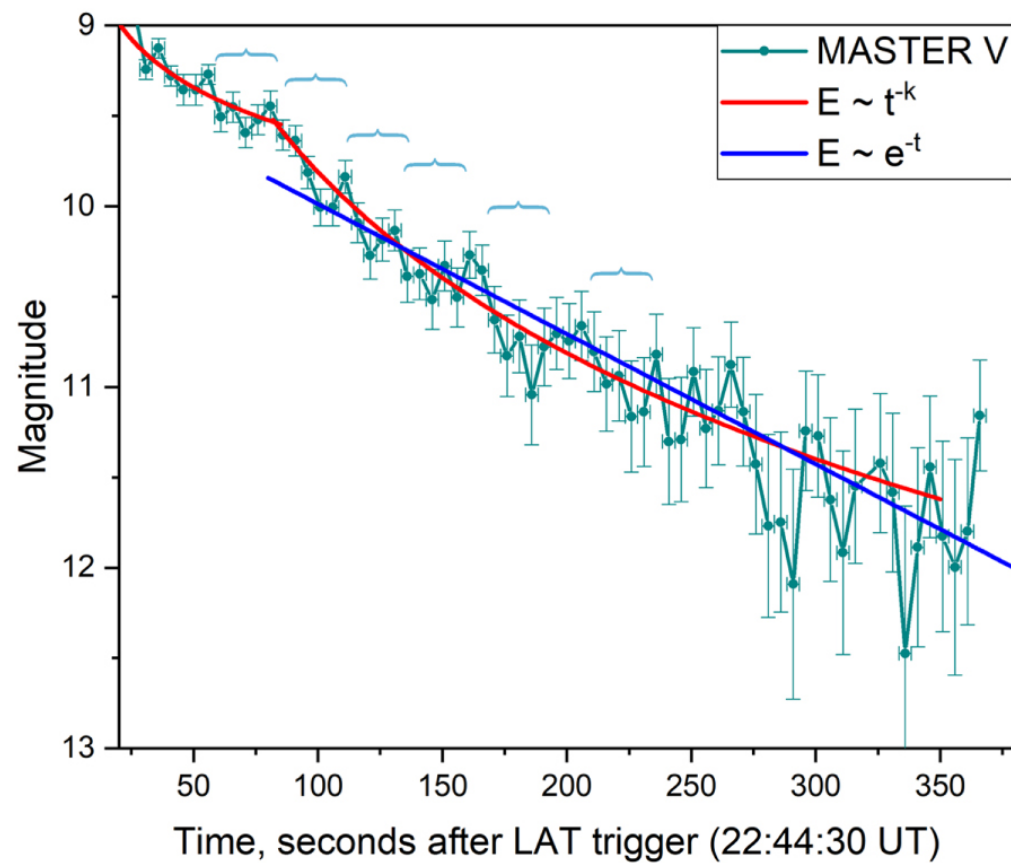
Figure 8. from V. M. Lipunov et al 2023 Astrophys. J. 943 doi:10.3847/1538-4357/ac9307 https://dx.doi.org/10.3847/1538-4357/ac9307 © 2023. The Author(s). Published by the American Astronomical Society.
