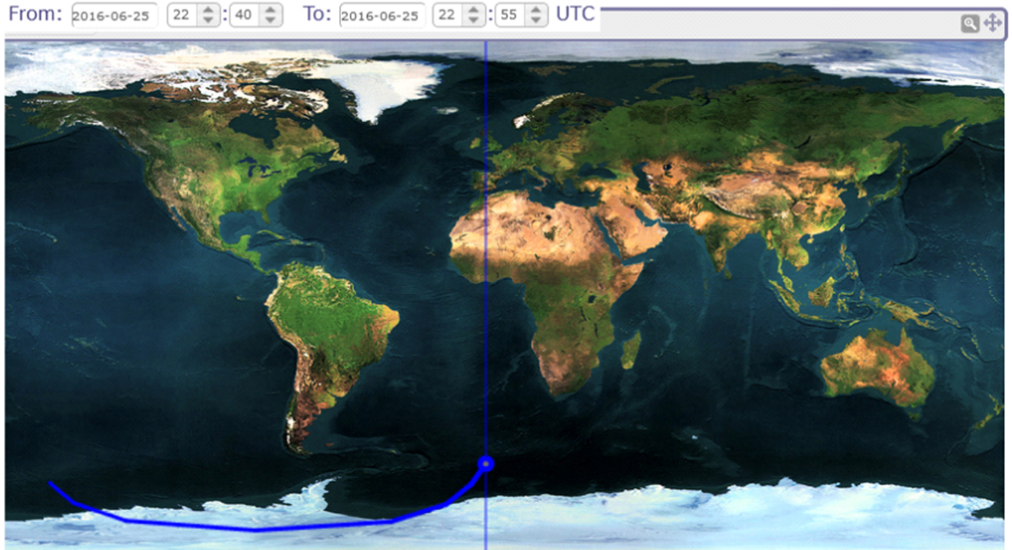
Figure 2. from V. M. Lipunov et al 2023 Astrophys. J. 943 doi:10.3847/1538-4357/ac9307 https://dx.doi.org/10.3847/1538-4357/ac9307 © 2023. The Author(s). Published by the American Astronomical Society.
