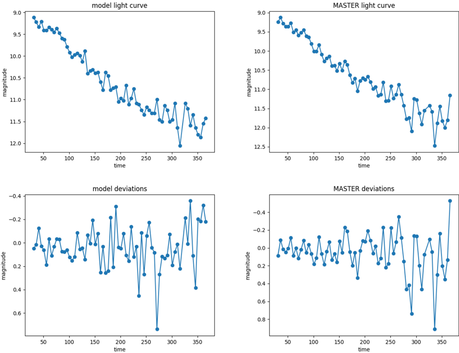
Figure 12. from V. M. Lipunov et al 2023 Astrophys. J. 943 doi:10.3847/1538-4357/ac9307 https://dx.doi.org/10.3847/1538-4357/ac9307 © 2023. The Author(s). Published by the American Astronomical Society.
