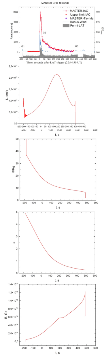
Figure 11. from V. M. Lipunov et al 2023 Astrophys. J. 943 doi:10.3847/1538-4357/ac9307 https://dx.doi.org/10.3847/1538-4357/ac9307 © 2023. The Author(s). Published by the American Astronomical Society.
