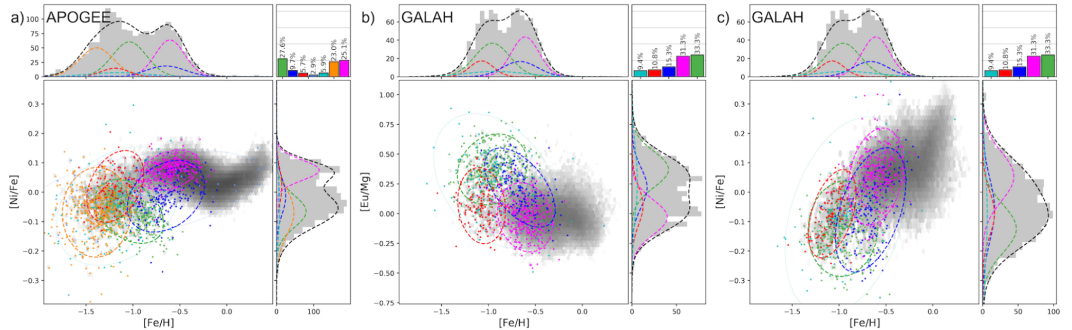
Figure 5. from G. C. Myeong et al 2022 Astrophys. J. 938 doi:10.3847/1538-4357/ac8d68 https://dx.doi.org/10.3847/1538-4357/ac8d68 © 2022. The Author(s). Published by the American Astronomical Society.
