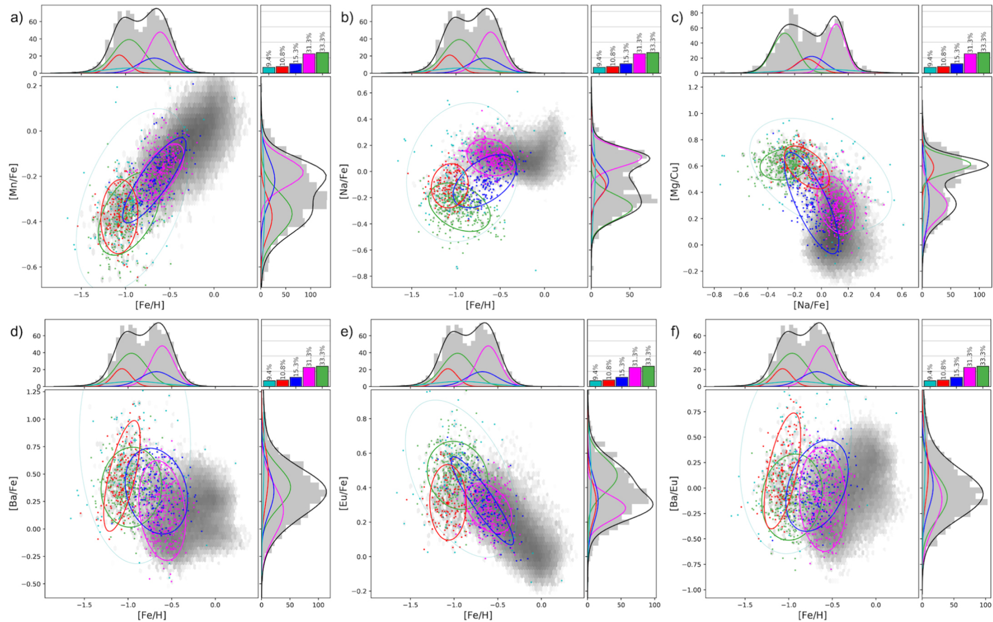
Figure 4. from G. C. Myeong et al 2022 Astrophys. J. 938 doi:10.3847/1538-4357/ac8d68 https://dx.doi.org/10.3847/1538-4357/ac8d68 © 2022. The Author(s). Published by the American Astronomical Society.
