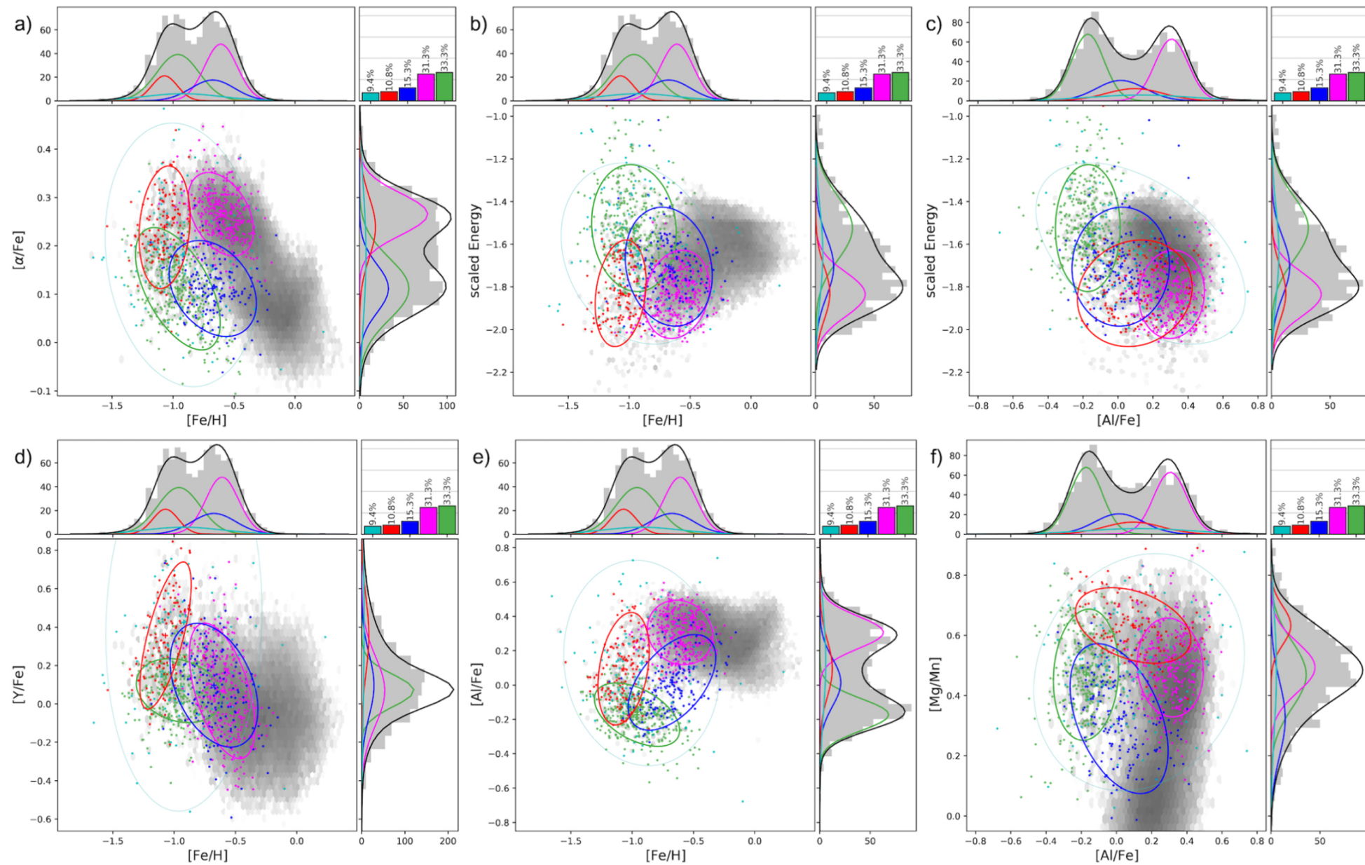
Figure 3. from G. C. Myeong et al 2022 Astrophys. J. 938 doi:10.3847/1538-4357/ac8d68 https://dx.doi.org/10.3847/1538-4357/ac8d68 © 2022. The Author(s). Published by the American Astronomical Society.
