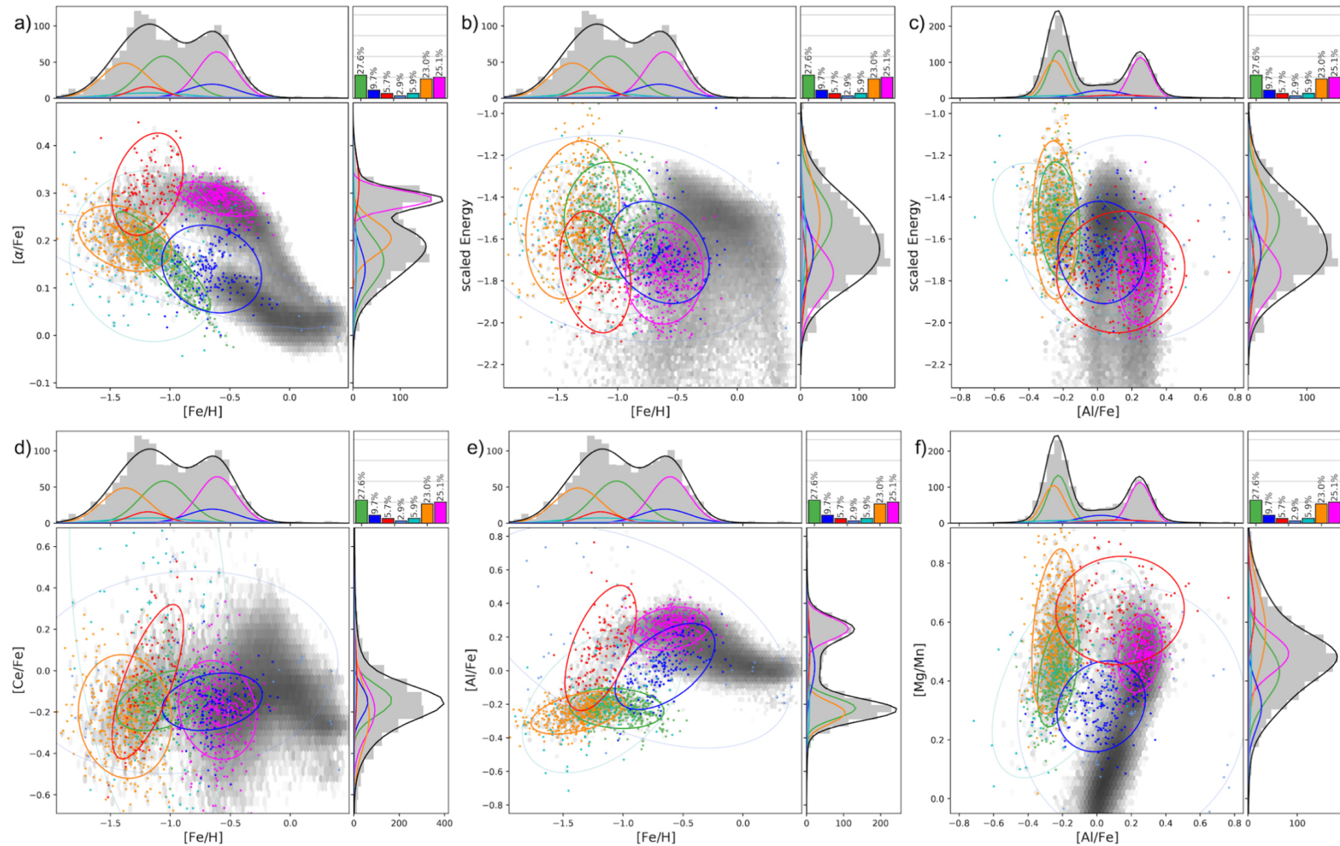
Figure 2. from G. C. Myeong et al 2022 Astrophys. J. 938 doi:10.3847/1538-4357/ac8d68 https://dx.doi.org/10.3847/1538-4357/ac8d68 © 2022. The Author(s). Published by the American Astronomical Society.
