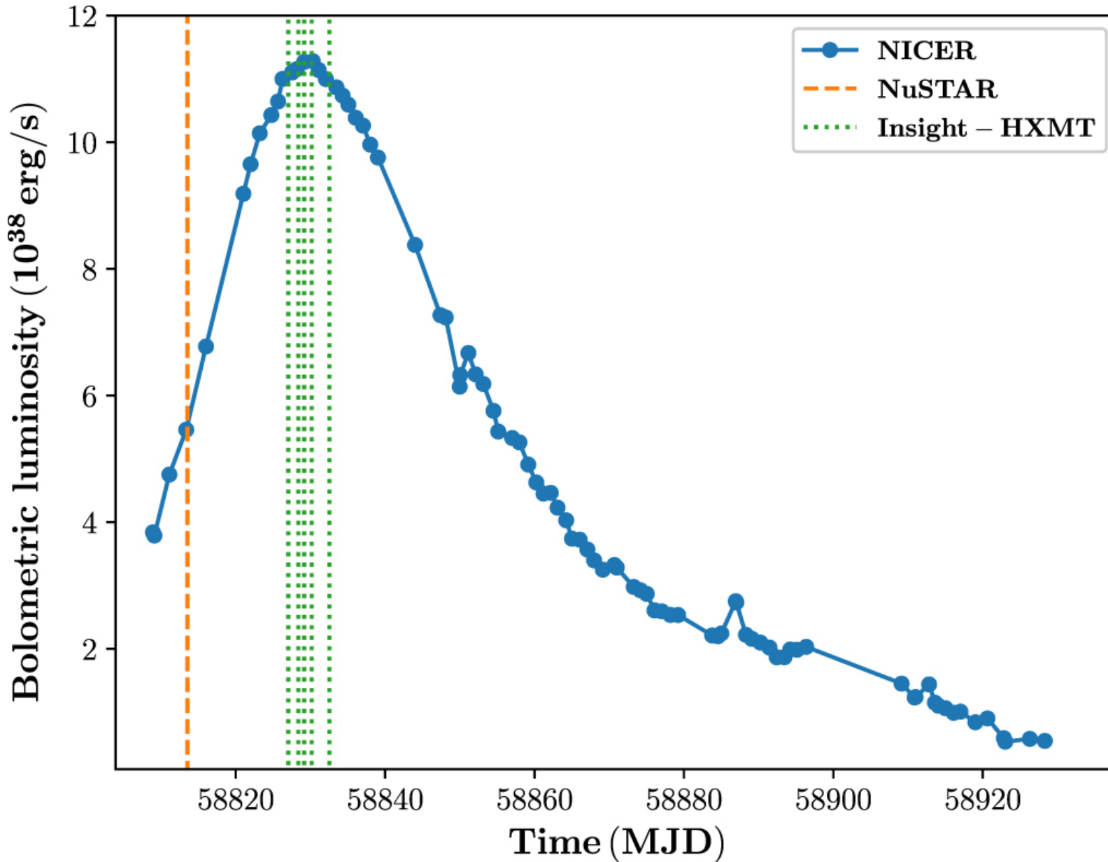
Figure 1. from X. Hou et al 2022 Astrophys. J. 938 doi:10.3847/1538-4357/ac8c93 https://dx.doi.org/10.3847/1538-4357/ac8c93 © 2022. The Author(s). Published by the American Astronomical Society.
