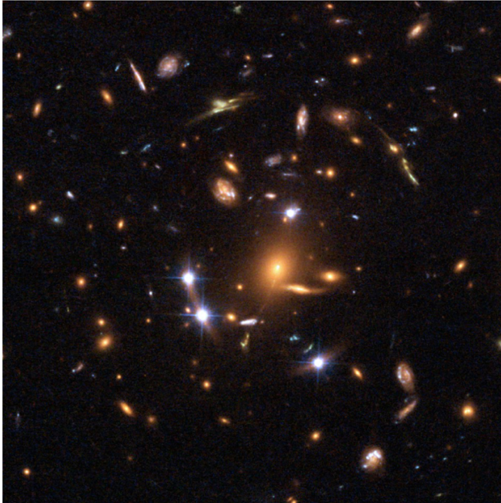
Figure 3. from R. Forés-Toribio et al 2022 Astrophys. J. 937 doi:10.3847/1538-4357/ac8c40 https://dx.doi.org/10.3847/1538-4357/ac8c40 © 2022. The Author(s). Published by the American Astronomical Society.
