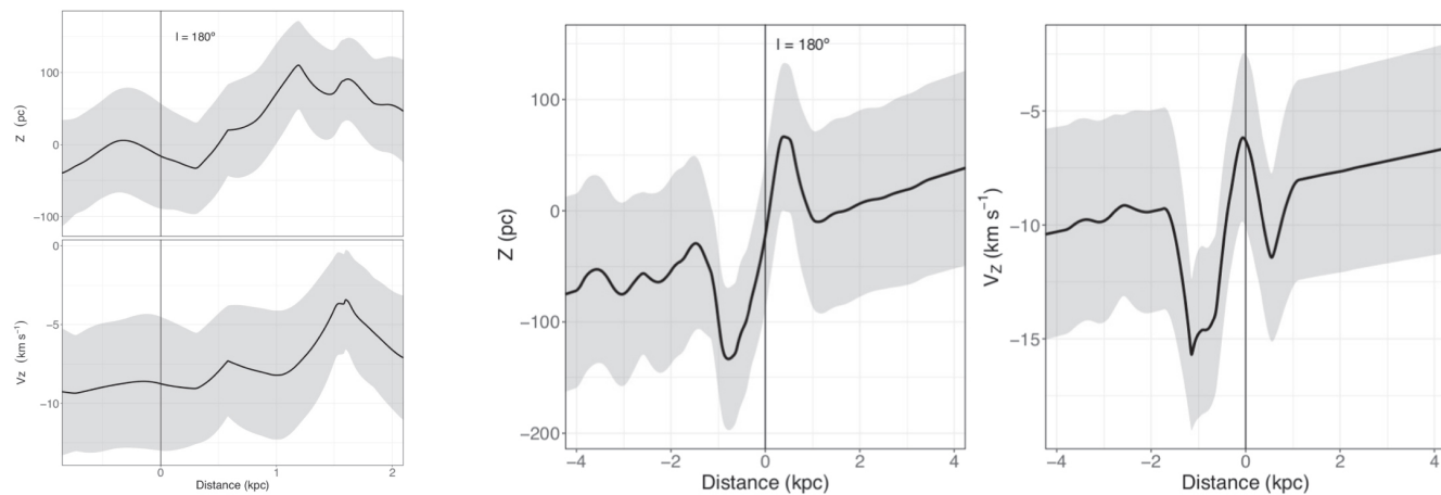
(b) Profiles along the Cepheus spur.
