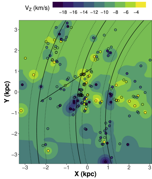
Figure 7. from Emilio J. Alfaro et al 2022 Astrophys. J. 937 doi:10.3847/1538-4357/ac8b0c https://dx.doi.org/10.3847/1538-4357/ac8b0c © 2022. The Author(s). Published by the American Astronomical Society.
