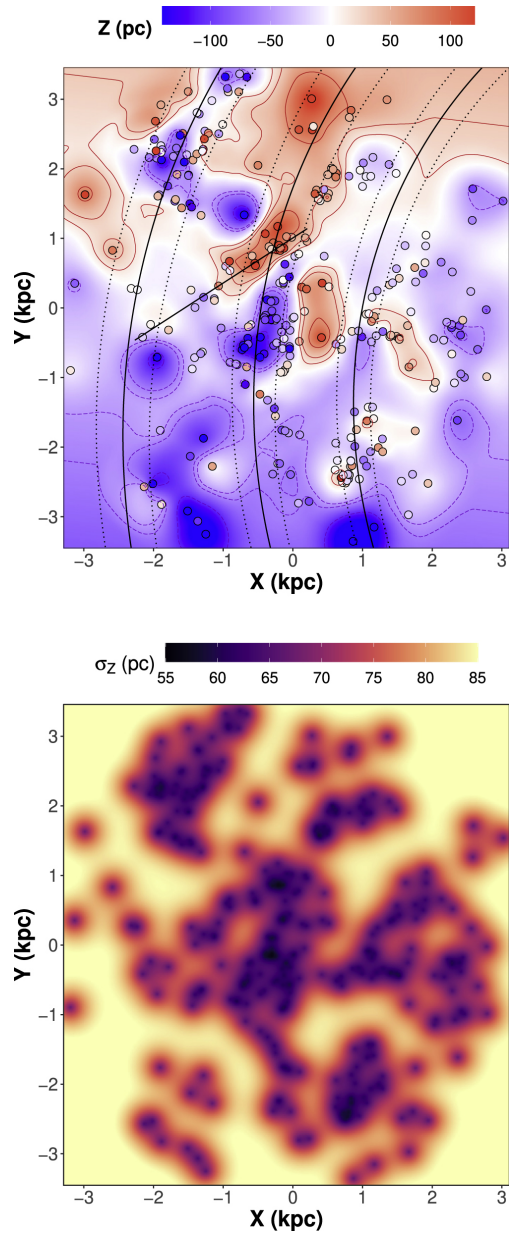
Figure 6. from Emilio J. Alfaro et al 2022 Astrophys. J. 937 doi:10.3847/1538-4357/ac8b0c https://dx.doi.org/10.3847/1538-4357/ac8b0c © 2022. The Author(s). Published by the American Astronomical Society.
