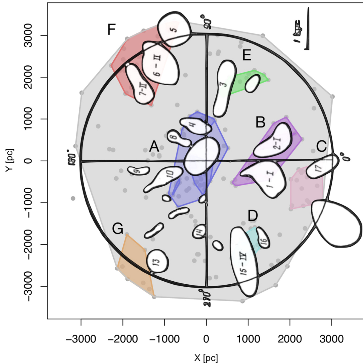
Figure 5. from Emilio J. Alfaro et al 2022 Astrophys. J. 937 doi:10.3847/1538-4357/ac8b0c https://dx.doi.org/10.3847/1538-4357/ac8b0c © 2022. The Author(s). Published by the American Astronomical Society.
