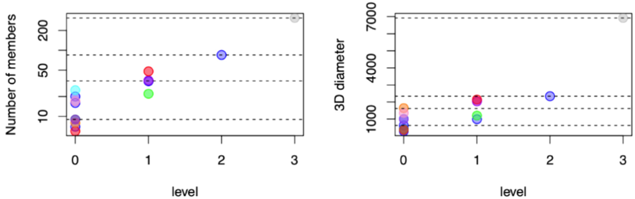
Figure 4. from Emilio J. Alfaro et al 2022 Astrophys. J. 937 doi:10.3847/1538-4357/ac8b0c https://dx.doi.org/10.3847/1538-4357/ac8b0c © 2022. The Author(s). Published by the American Astronomical Society.
