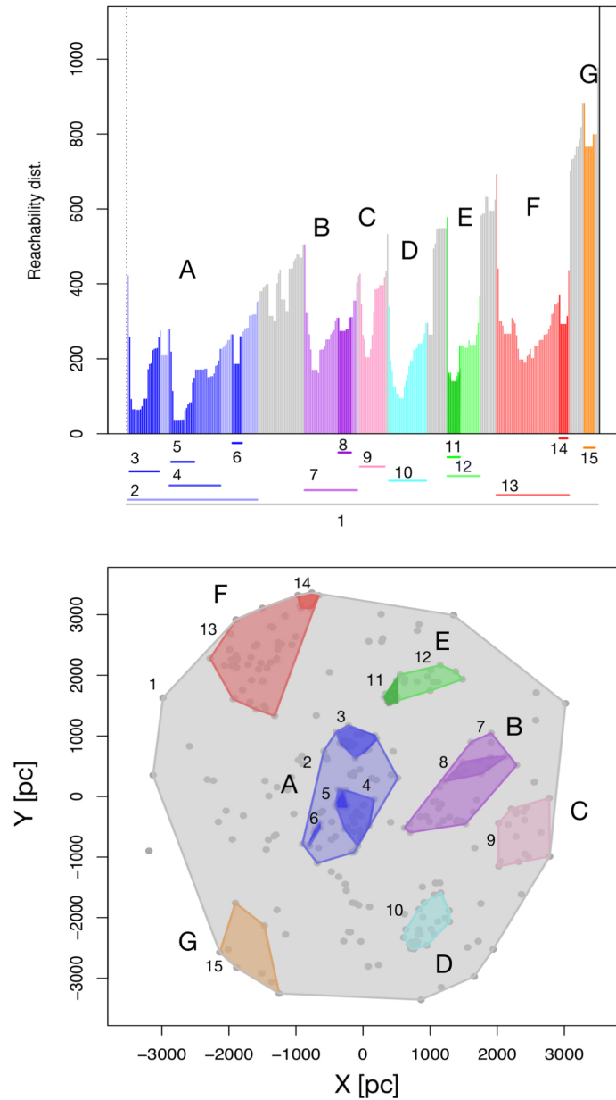
Figure 3. from Emilio J. Alfaro et al 2022 Astrophys. J. 937 doi:10.3847/1538-4357/ac8b0c https://dx.doi.org/10.3847/1538-4357/ac8b0c © 2022. The Author(s). Published by the American Astronomical Society.
