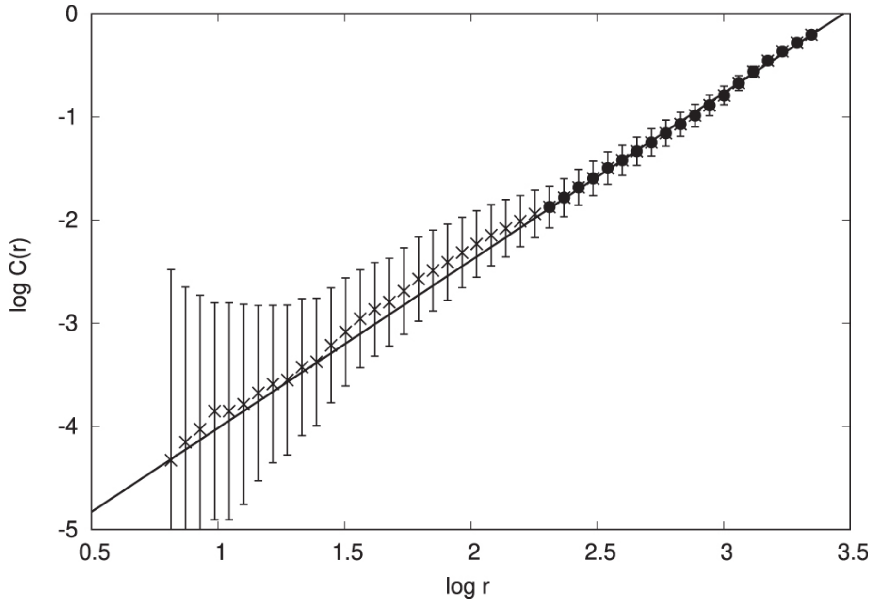
Figure 2. from Emilio J. Alfaro et al 2022 Astrophys. J. 937 doi:10.3847/1538-4357/ac8b0c https://dx.doi.org/10.3847/1538-4357/ac8b0c © 2022. The Author(s). Published by the American Astronomical Society.
