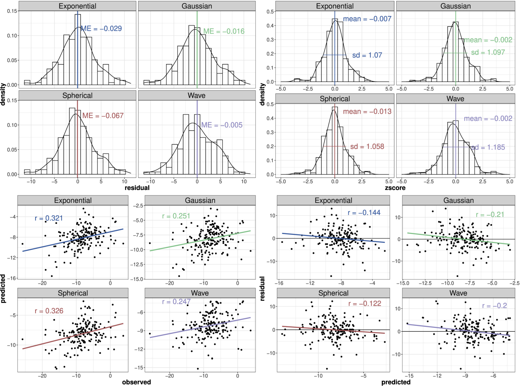
Figure 17. from Emilio J. Alfaro et al 2022 Astrophys. J. 937 doi:10.3847/1538-4357/ac8b0c https://dx.doi.org/10.3847/1538-4357/ac8b0c © 2022. The Author(s). Published by the American Astronomical Society.
