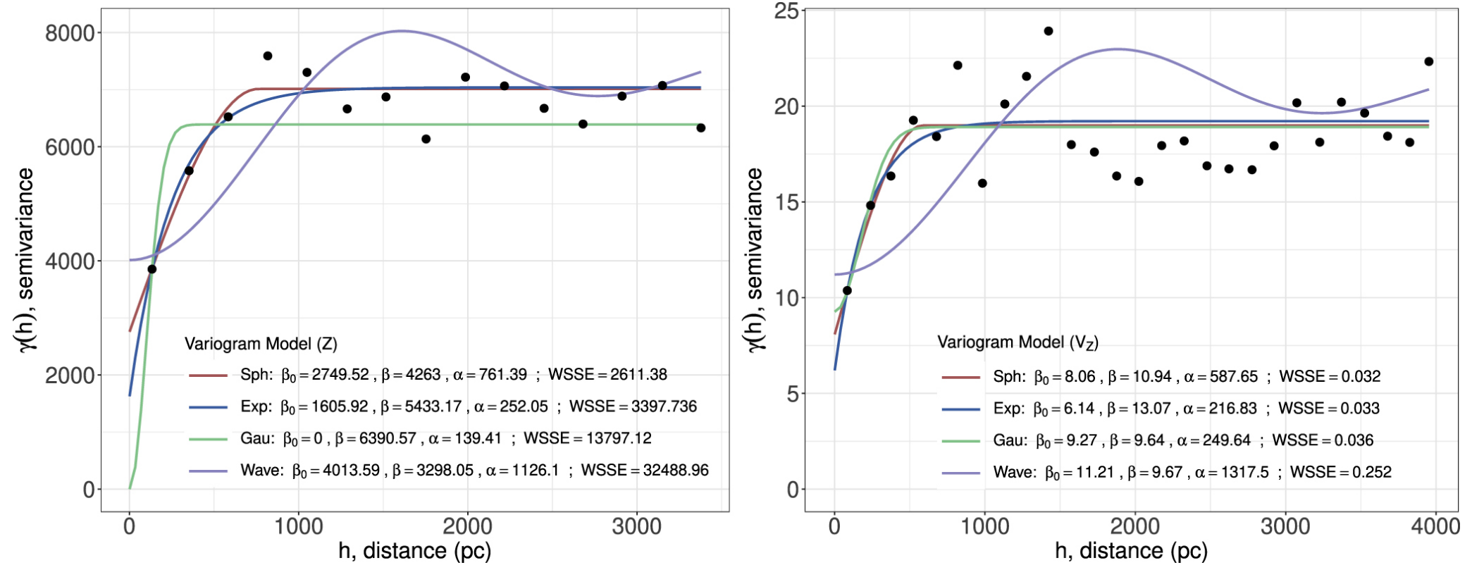
Figure 15. from Emilio J. Alfaro et al 2022 Astrophys. J. 937 doi:10.3847/1538-4357/ac8b0c https://dx.doi.org/10.3847/1538-4357/ac8b0c © 2022. The Author(s). Published by the American Astronomical Society.
