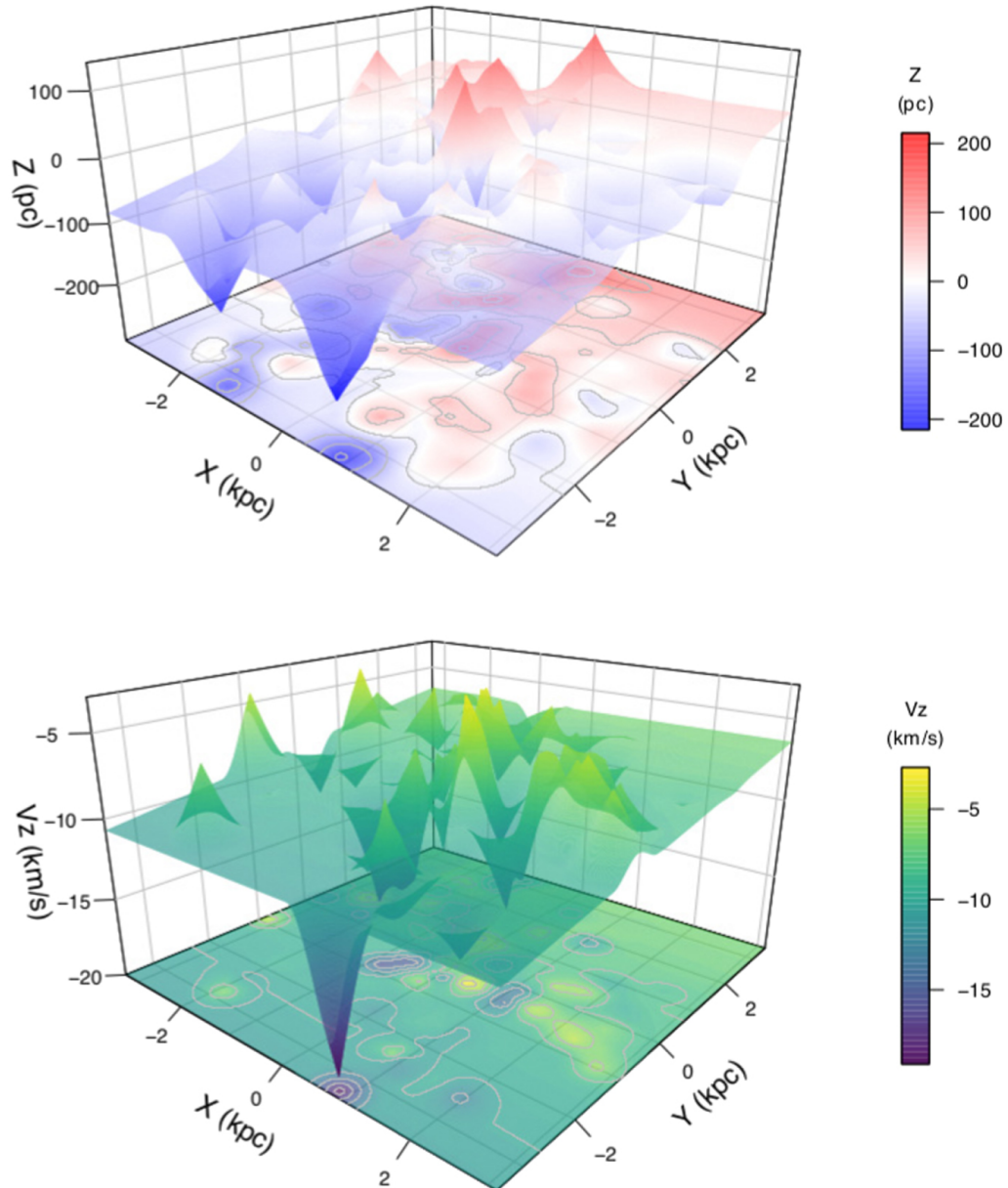
Figure 14. from Emilio J. Alfaro et al 2022 Astrophys. J. 937 doi:10.3847/1538-4357/ac8b0c https://dx.doi.org/10.3847/1538-4357/ac8b0c © 2022. The Author(s). Published by the American Astronomical Society.
