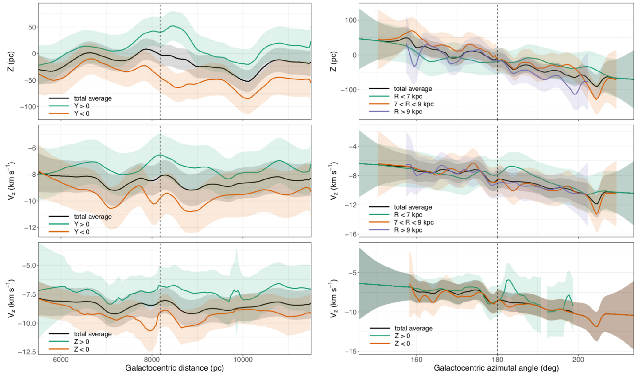
Figure 11. from Emilio J. Alfaro et al 2022 Astrophys. J. 937 doi:10.3847/1538-4357/ac8b0c https://dx.doi.org/10.3847/1538-4357/ac8b0c © 2022. The Author(s). Published by the American Astronomical Society.
