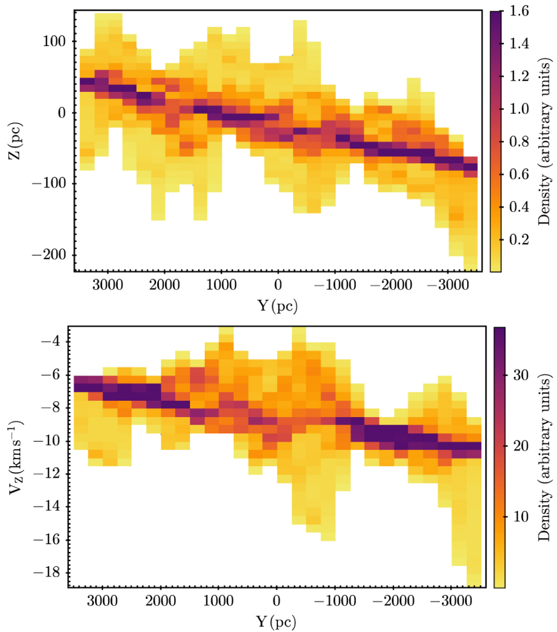
Figure 10. from Emilio J. Alfaro et al 2022 Astrophys. J. 937 doi:10.3847/1538-4357/ac8b0c https://dx.doi.org/10.3847/1538-4357/ac8b0c © 2022. The Author(s). Published by the American Astronomical Society.
