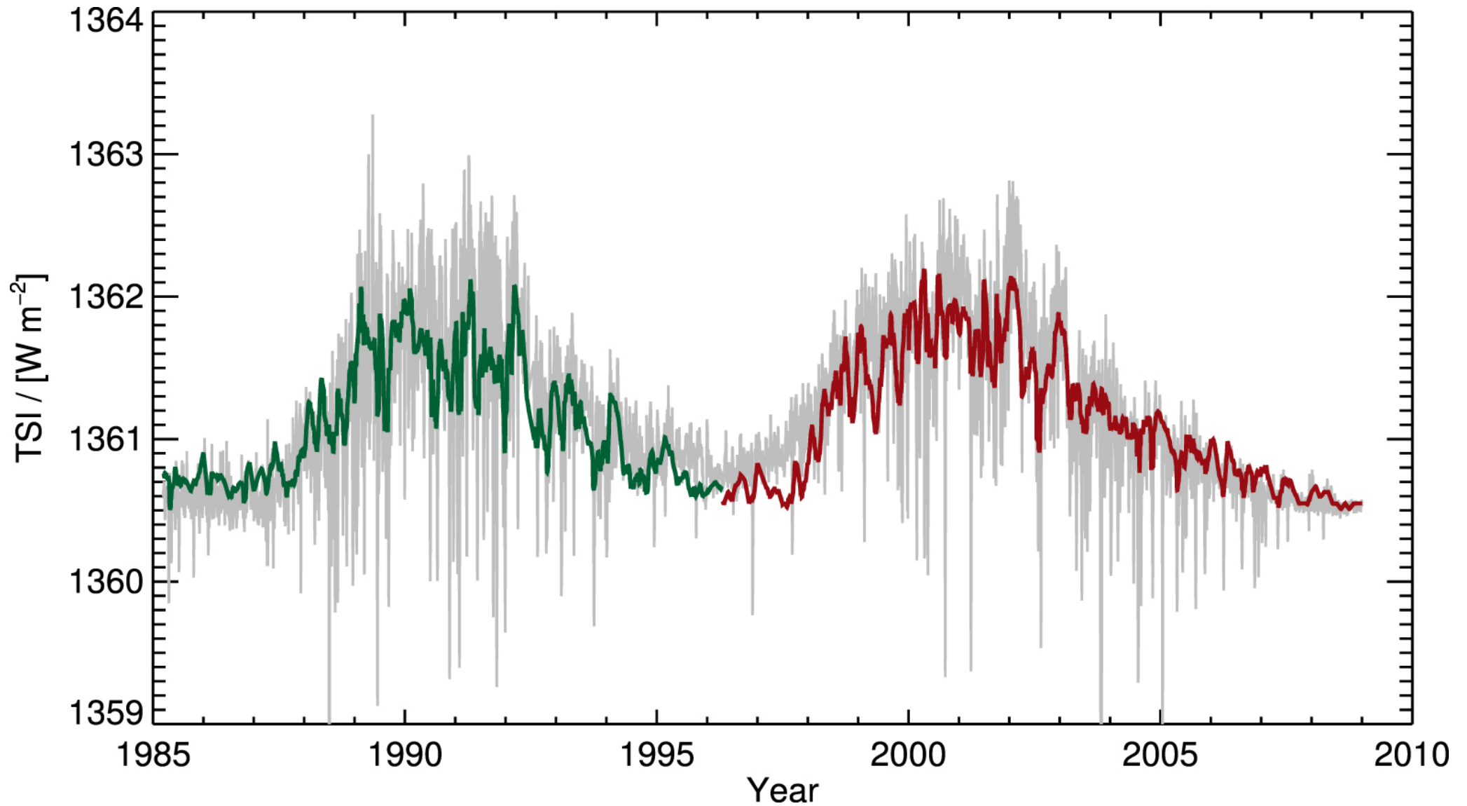
Figure 9. from Valentina Penza et al 2022 Astrophys. J. 937 doi:10.3847/1538-4357/ac8a4b https://dx.doi.org/10.3847/1538-4357/ac8a4b © 2022. The Author(s). Published by the American Astronomical Society.
