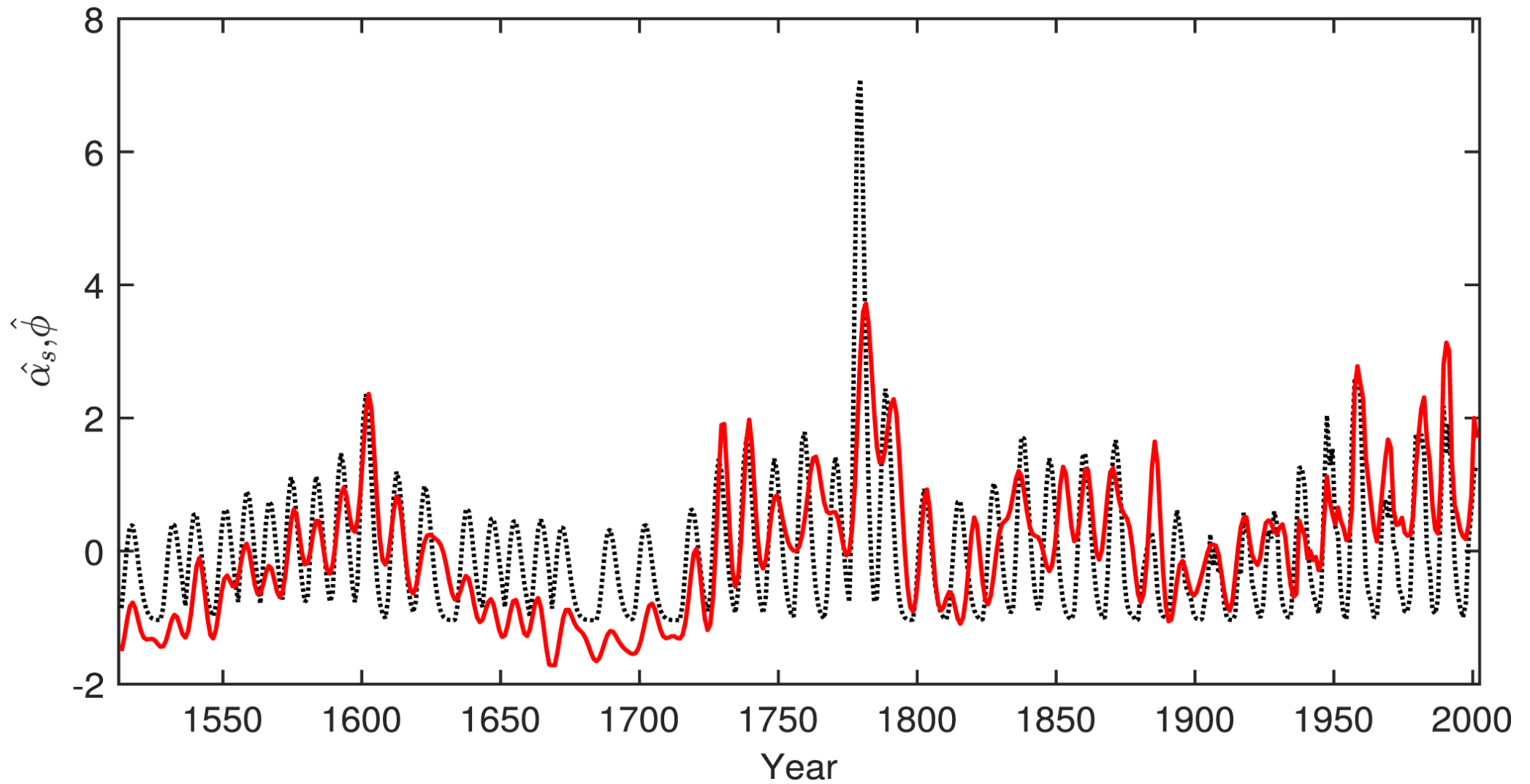
Figure 7. from Valentina Penza et al 2022 Astrophys. J. 937 doi:10.3847/1538-4357/ac8a4b https://dx.doi.org/10.3847/1538-4357/ac8a4b © 2022. The Author(s). Published by the American Astronomical Society.
