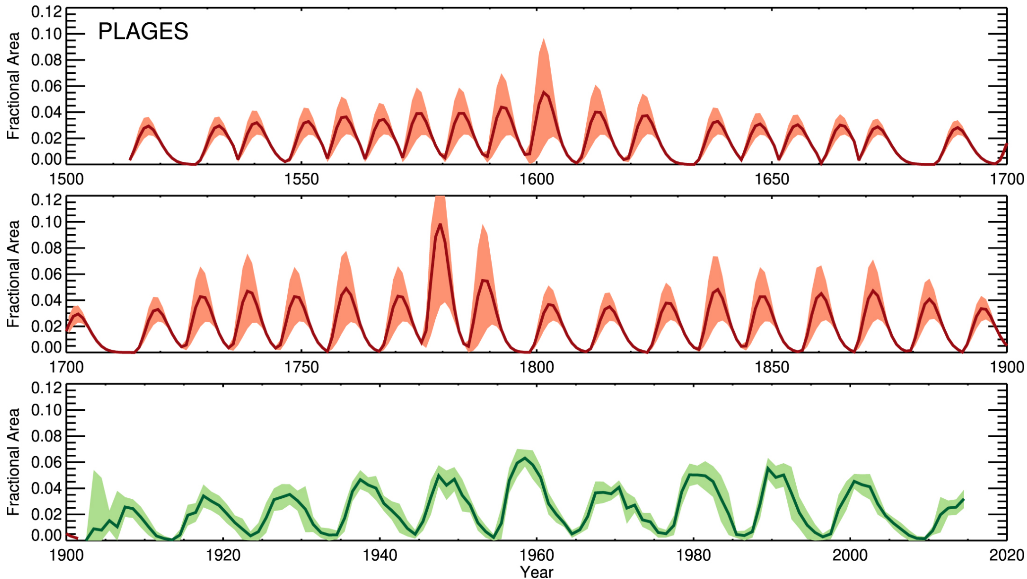
Figure 5. from Valentina Penza et al 2022 Astrophys. J. 937 doi:10.3847/1538-4357/ac8a4b https://dx.doi.org/10.3847/1538-4357/ac8a4b © 2022. The Author(s). Published by the American Astronomical Society.
