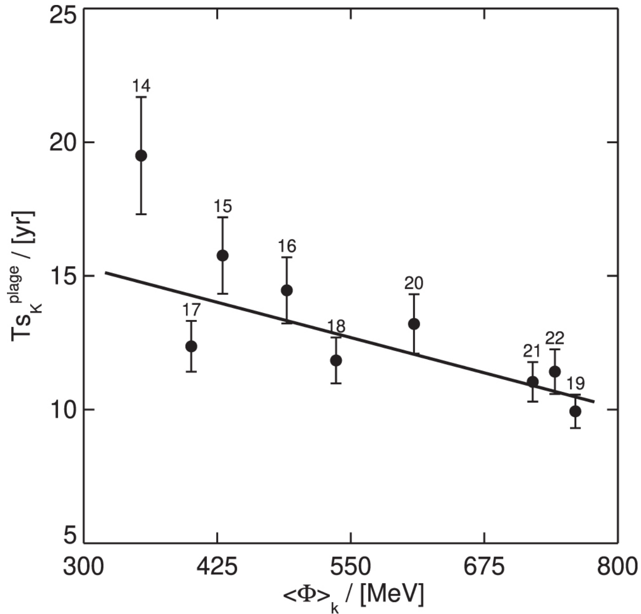
Figure 4. from Valentina Penza et al 2022 Astrophys. J. 937 doi:10.3847/1538-4357/ac8a4b https://dx.doi.org/10.3847/1538-4357/ac8a4b © 2022. The Author(s). Published by the American Astronomical Society.
