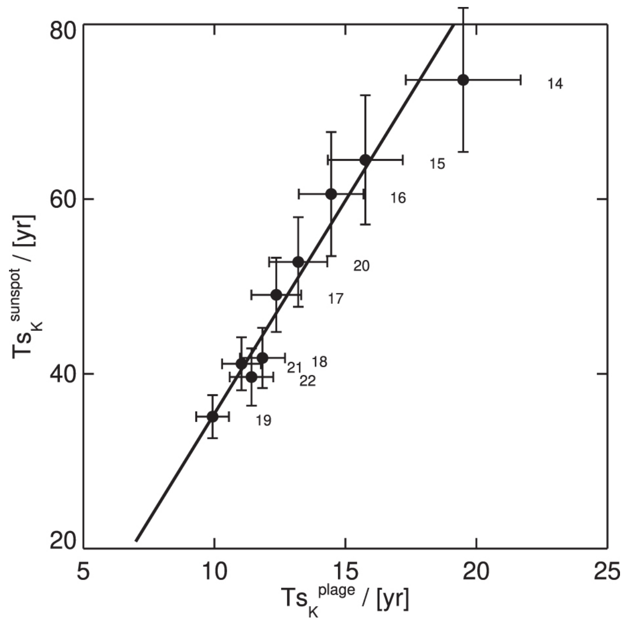
Figure 3. from Valentina Penza et al 2022 Astrophys. J. 937 doi:10.3847/1538-4357/ac8a4b https://dx.doi.org/10.3847/1538-4357/ac8a4b © 2022. The Author(s). Published by the American Astronomical Society.
