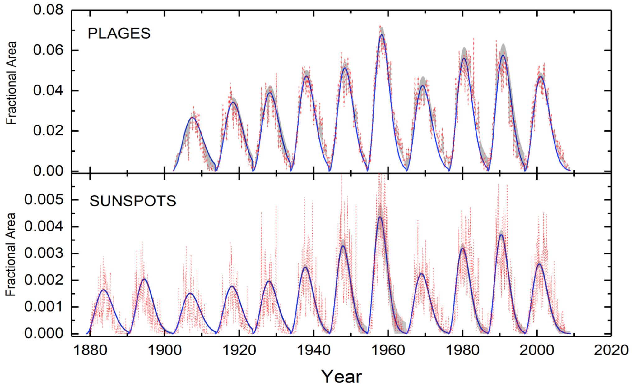
Figure 2. from Valentina Penza et al 2022 Astrophys. J. 937 doi:10.3847/1538-4357/ac8a4b https://dx.doi.org/10.3847/1538-4357/ac8a4b © 2022. The Author(s). Published by the American Astronomical Society.
