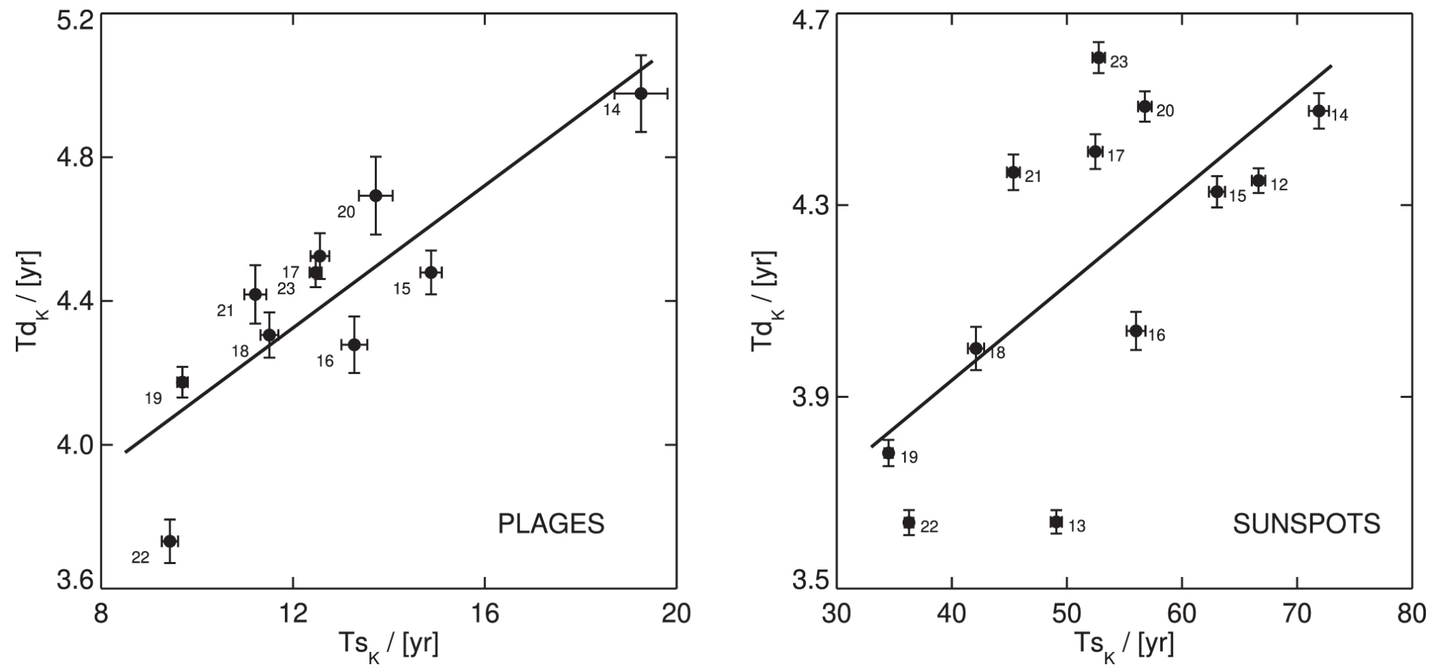
Figure 1. from Valentina Penza et al 2022 Astrophys. J. 937 doi:10.3847/1538-4357/ac8a4b https://dx.doi.org/10.3847/1538-4357/ac8a4b © 2022. The Author(s). Published by the American Astronomical Society.
