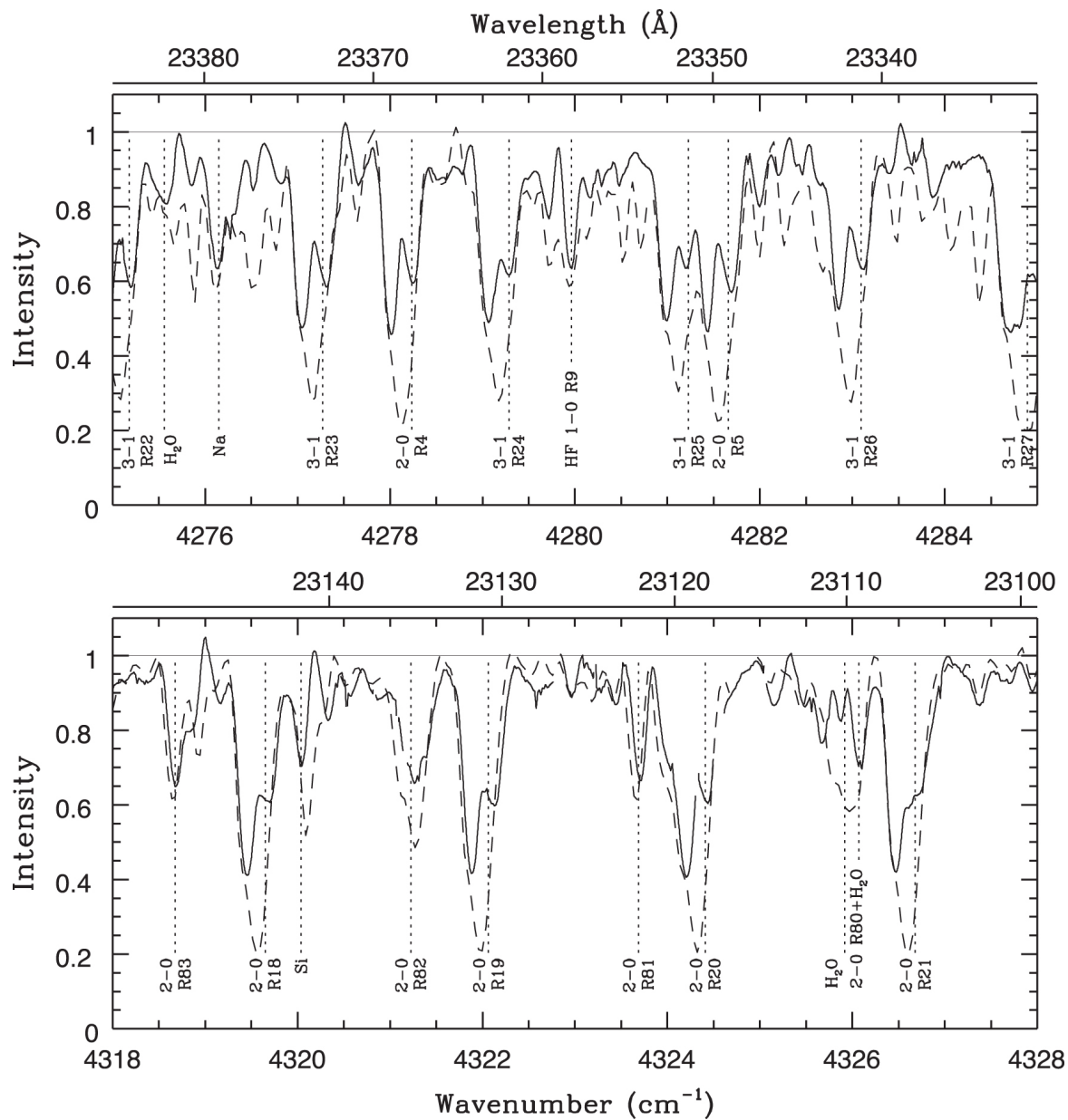
Figure 9. from Kenneth H. Hinkle et al 2022 Astrophys. J. 937 doi:10.3847/1538-4357/ac8a47 https://dx.doi.org/10.3847/1538-4357/ac8a47 © 2022. The Author(s). Published by the American Astronomical Society.
