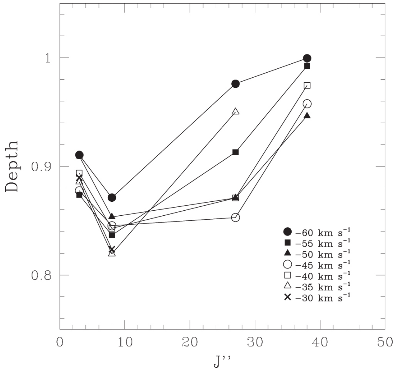
Figure 8. from Kenneth H. Hinkle et al 2022 Astrophys. J. 937 doi:10.3847/1538-4357/ac8a47 https://dx.doi.org/10.3847/1538-4357/ac8a47 © 2022. The Author(s). Published by the American Astronomical Society.
