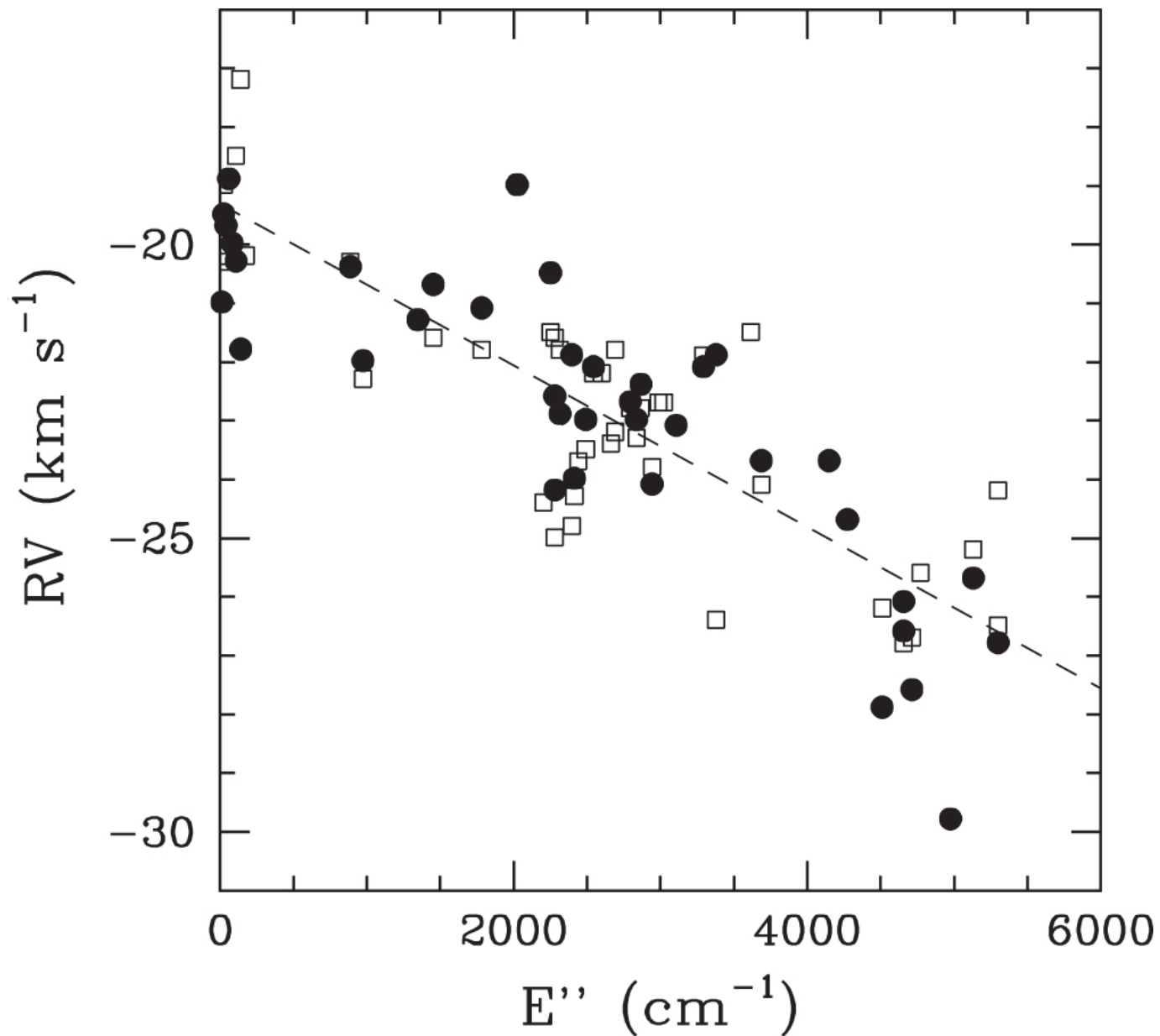
Figure 6. from Kenneth H. Hinkle et al 2022 Astrophys. J. 937 doi:10.3847/1538-4357/ac8a47 https://dx.doi.org/10.3847/1538-4357/ac8a47 © 2022. The Author(s). Published by the American Astronomical Society.
