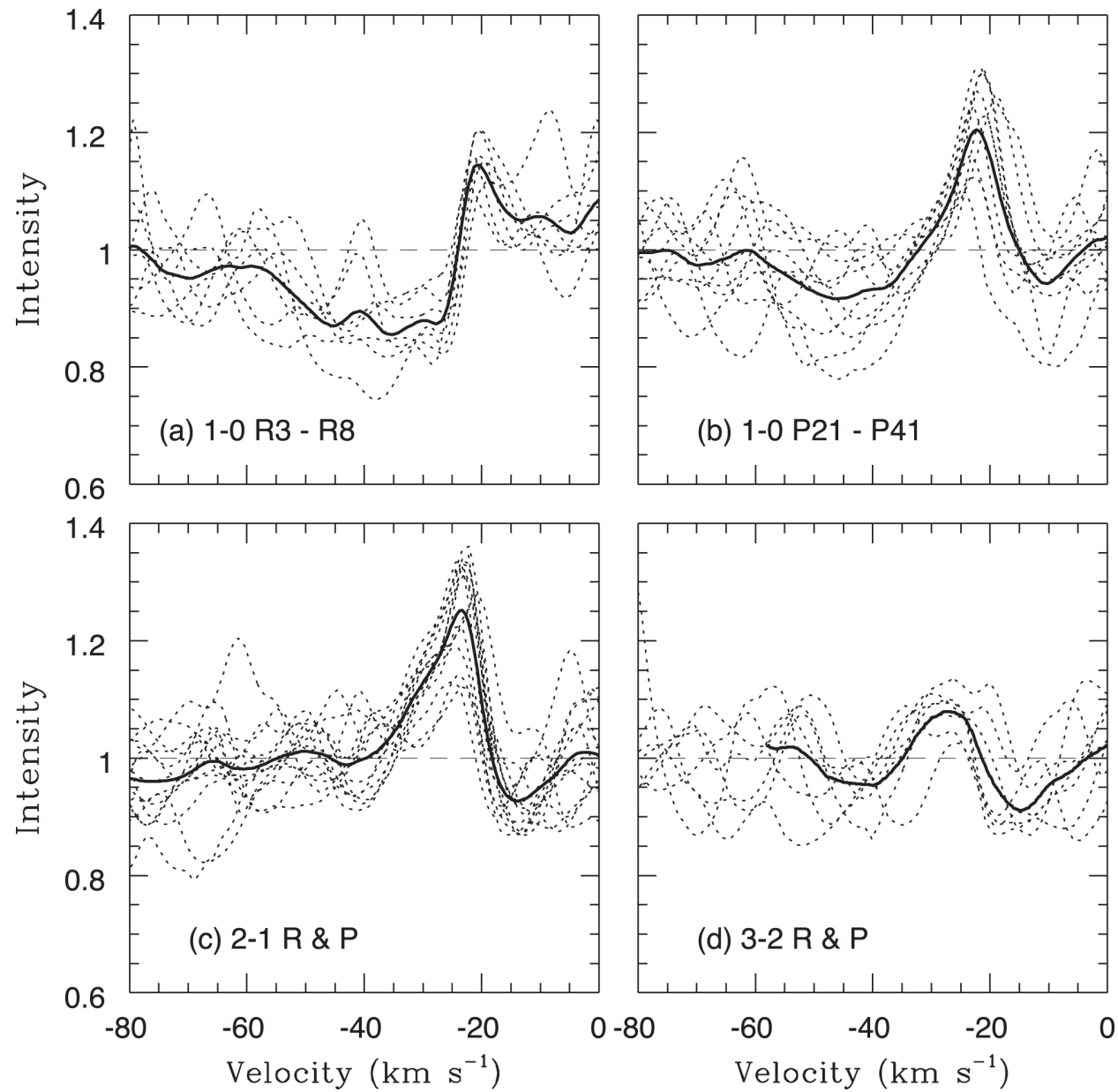
Figure 5. from Kenneth H. Hinkle et al 2022 Astrophys. J. 937 doi:10.3847/1538-4357/ac8a47 https://dx.doi.org/10.3847/1538-4357/ac8a47 © 2022. The Author(s). Published by the American Astronomical Society.
