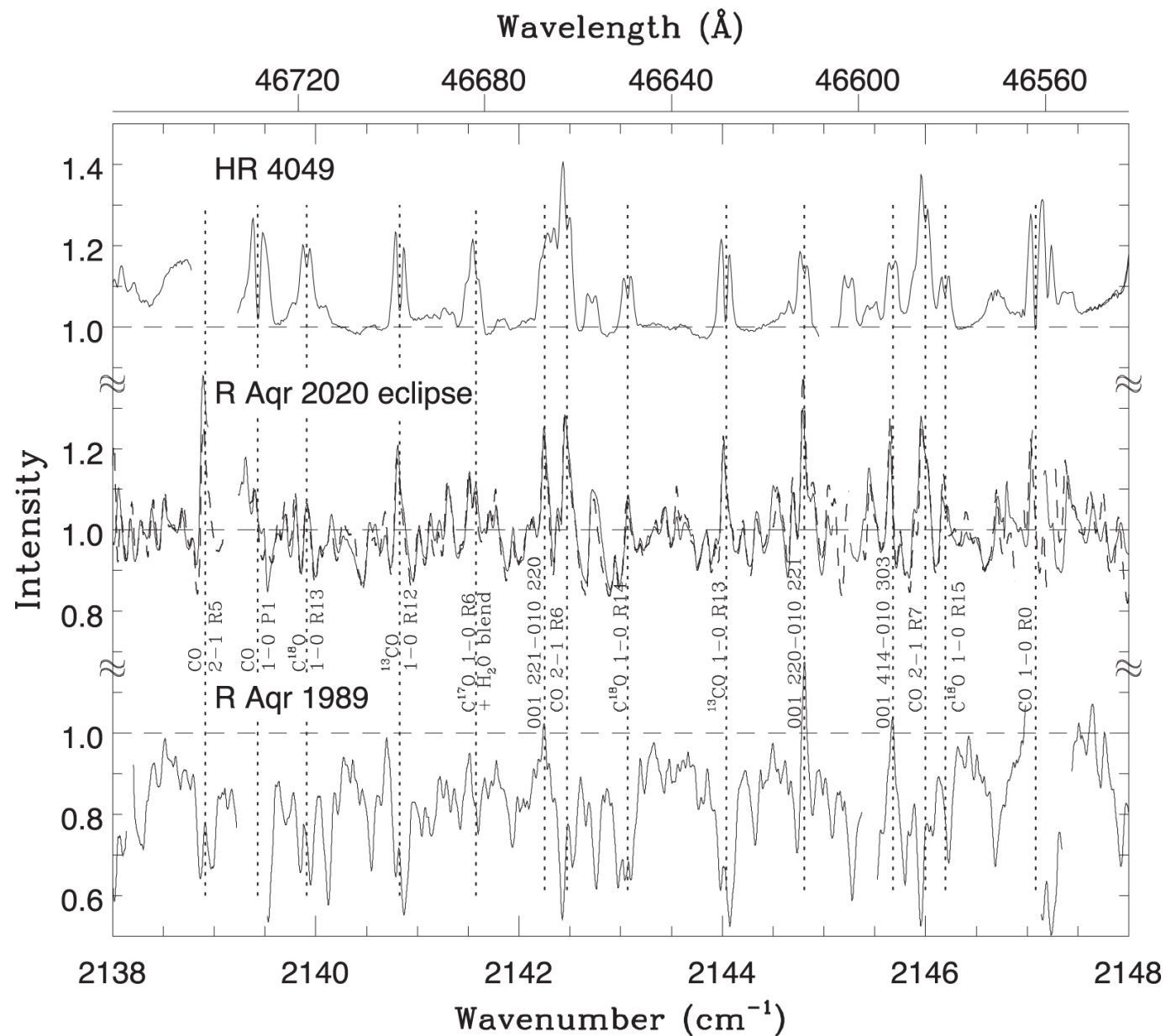
Figure 3. from Kenneth H. Hinkle et al 2022 Astrophys. J. 937 doi:10.3847/1538-4357/ac8a47 https://dx.doi.org/10.3847/1538-4357/ac8a47 © 2022. The Author(s). Published by the American Astronomical Society.
