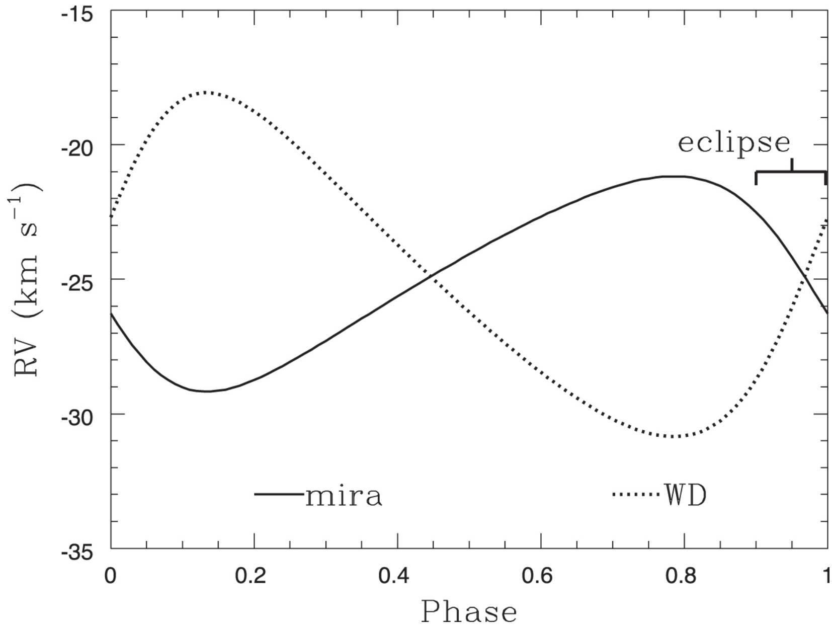
Figure 1. from Kenneth H. Hinkle et al 2022 Astrophys. J. 937 doi:10.3847/1538-4357/ac8a47 https://dx.doi.org/10.3847/1538-4357/ac8a47 © 2022. The Author(s). Published by the American Astronomical Society.
