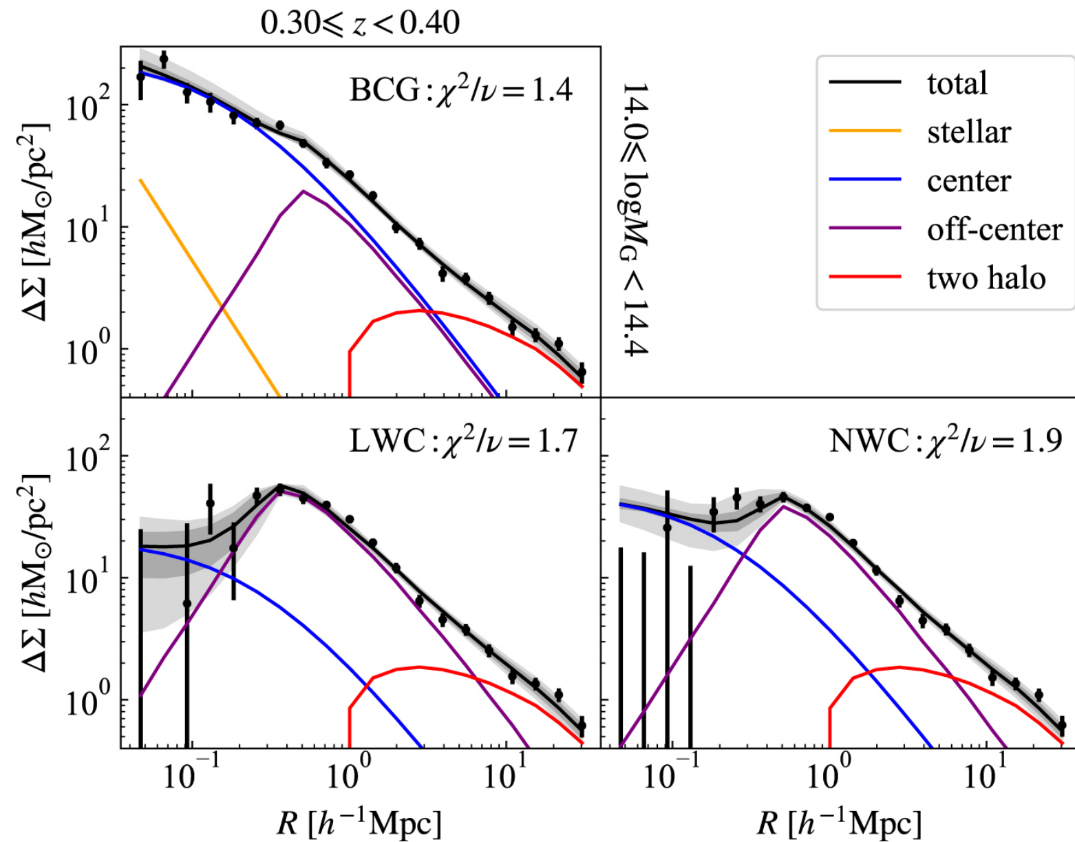
Figure 3. from Jiaqi Wang et al 2022 Astrophys. J. 936 doi:10.3847/1538-4357/ac8986 https://dx.doi.org/10.3847/1538-4357/ac8986 © 2022. The Author(s). Published by the American Astronomical Society.
