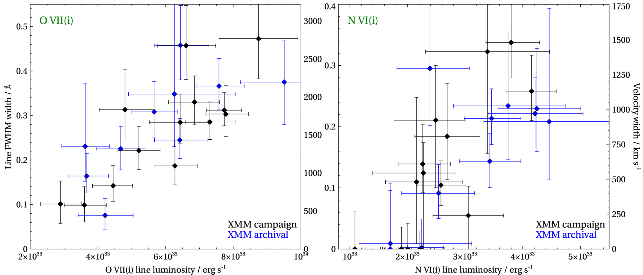
Figure 7. from P. Kosec et al 2022 Astrophys. J. 936 doi:10.3847/1538-4357/ac897e https://dx.doi.org/10.3847/1538-4357/ac897e © 2022. The Author(s). Published by the American Astronomical Society.
