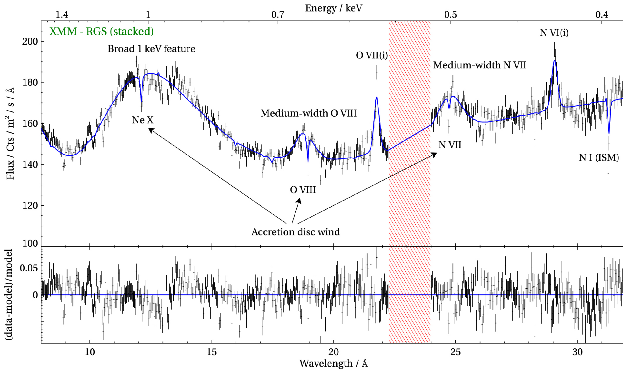
Figure 5. from P. Kosec et al 2022 Astrophys. J. 936 doi:10.3847/1538-4357/ac897e https://dx.doi.org/10.3847/1538-4357/ac897e © 2022. The Author(s). Published by the American Astronomical Society.
