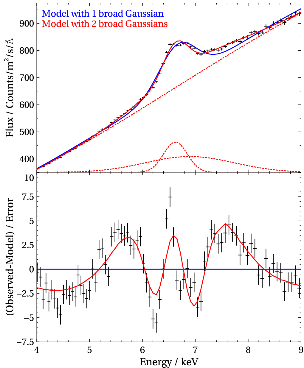
Figure 3. from P. Kosec et al 2022 Astrophys. J. 936 doi:10.3847/1538-4357/ac897e https://dx.doi.org/10.3847/1538-4357/ac897e © 2022. The Author(s). Published by the American Astronomical Society.
