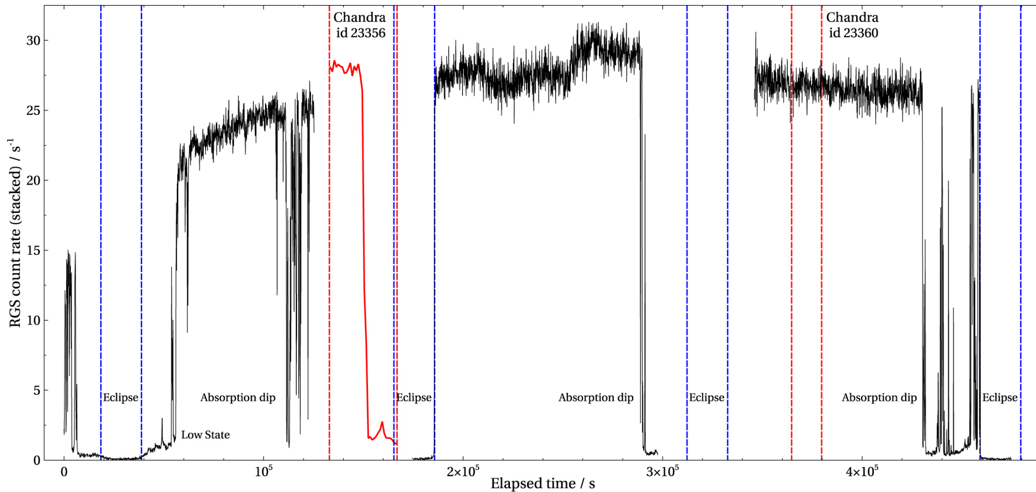
Figure 2. from P. Kosec et al 2022 Astrophys. J. 936 doi:10.3847/1538-4357/ac897e https://dx.doi.org/10.3847/1538-4357/ac897e © 2022. The Author(s). Published by the American Astronomical Society.
