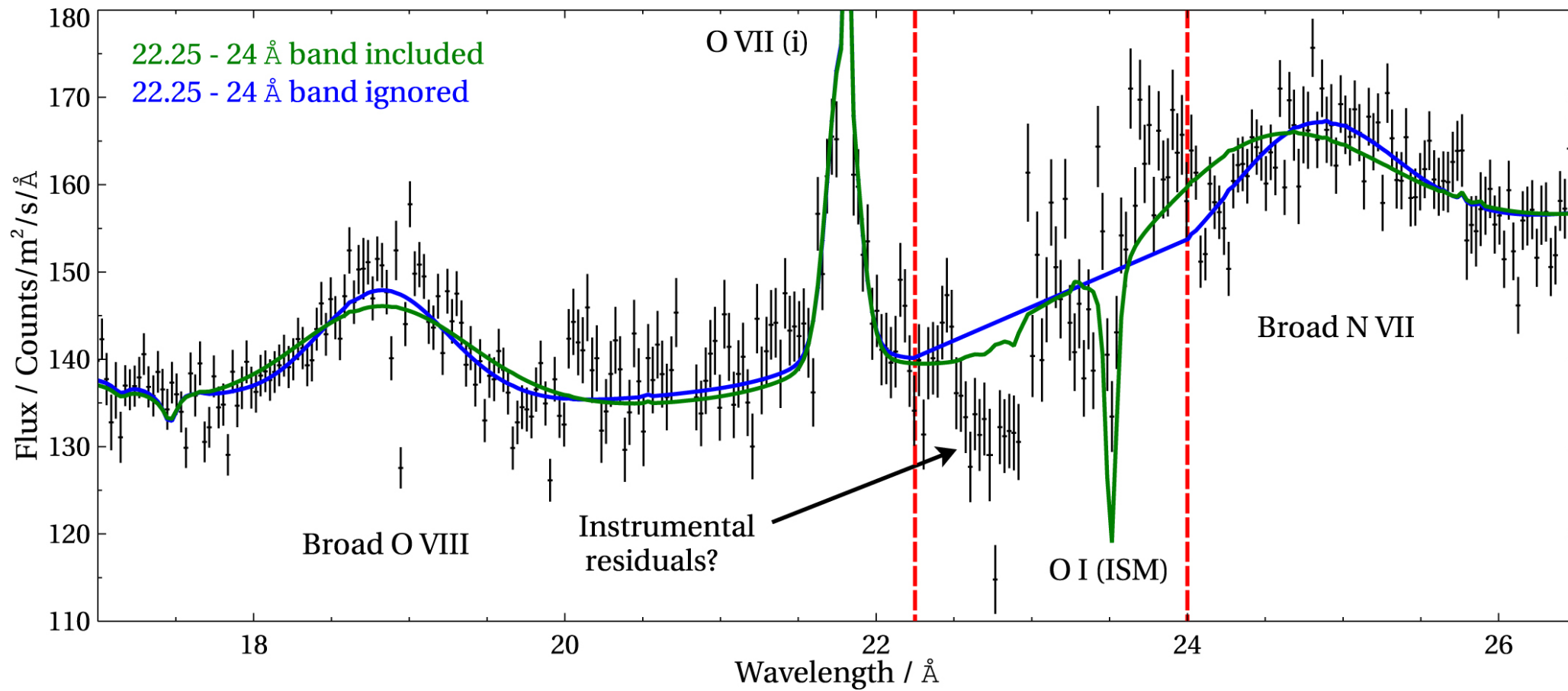
Figure 17. from P. Kosec et al 2022 Astrophys. J. 936 doi:10.3847/1538-4357/ac897e https://dx.doi.org/10.3847/1538-4357/ac897e © 2022. The Author(s). Published by the American Astronomical Society.
