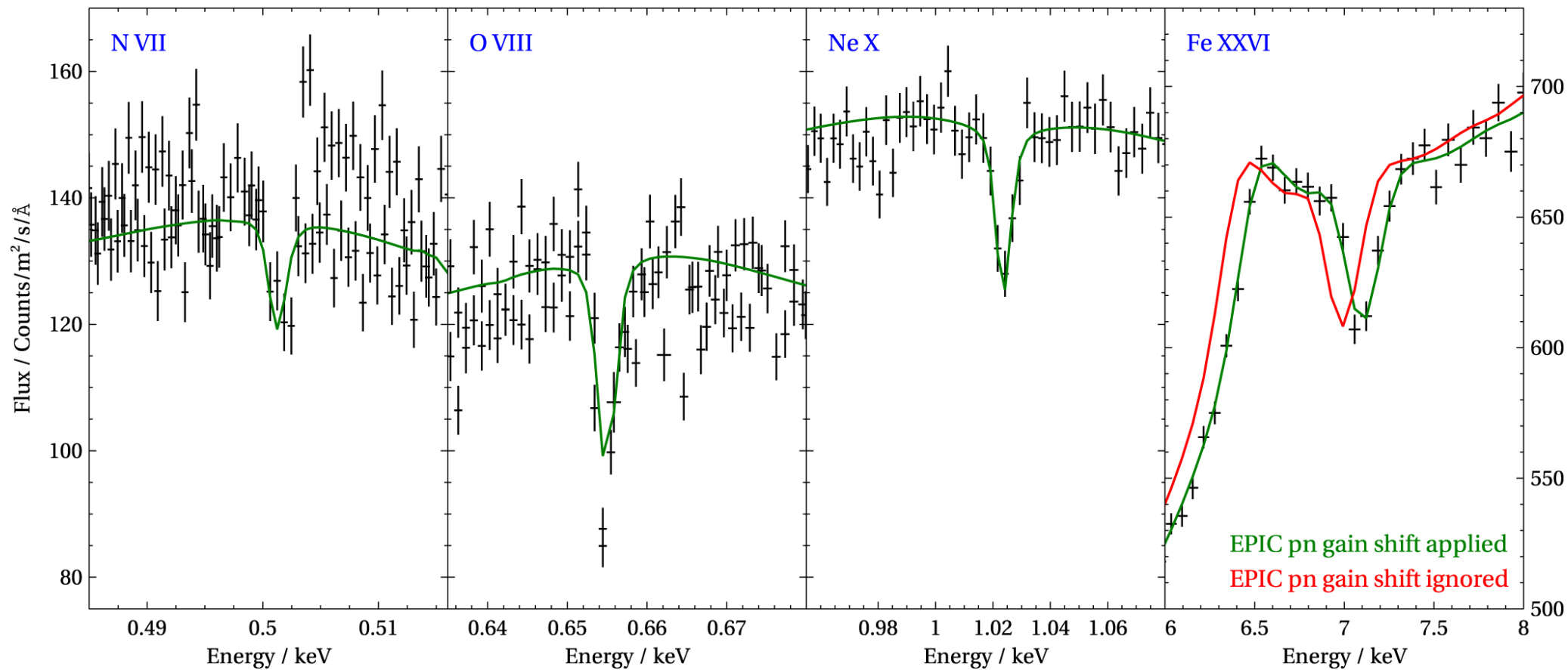
Figure 14. from P. Kosec et al 2022 Astrophys. J. 936 doi:10.3847/1538-4357/ac897e https://dx.doi.org/10.3847/1538-4357/ac897e © 2022. The Author(s). Published by the American Astronomical Society.
