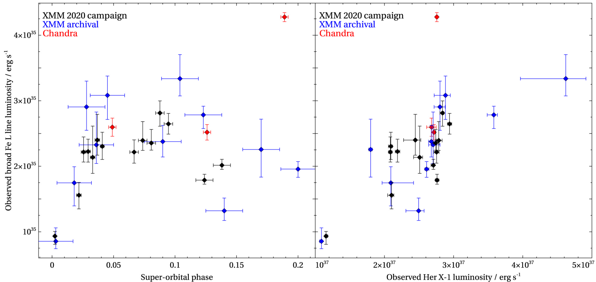
Figure 12. from P. Kosec et al 2022 Astrophys. J. 936 doi:10.3847/1538-4357/ac897e https://dx.doi.org/10.3847/1538-4357/ac897e © 2022. The Author(s). Published by the American Astronomical Society.
