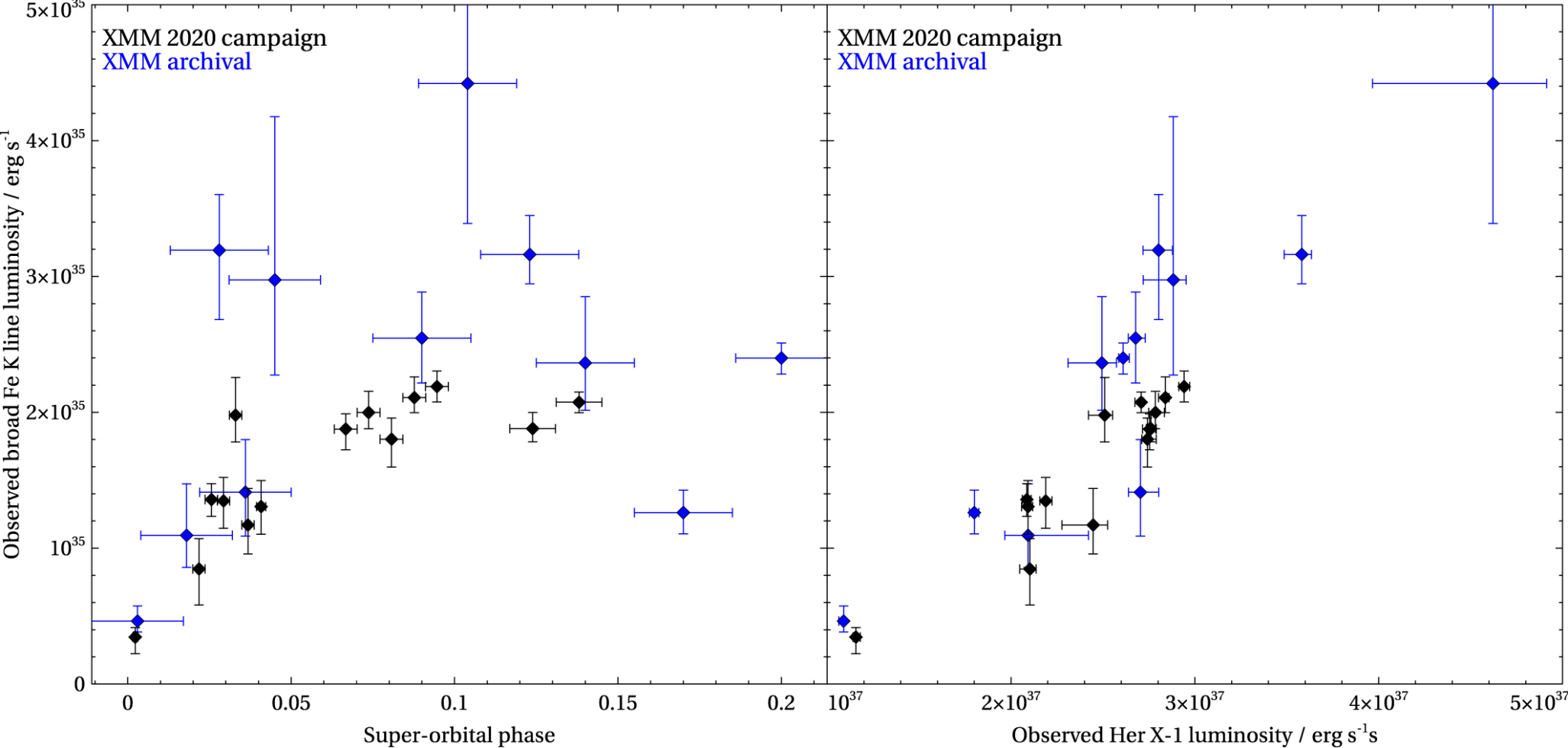
Figure 10. from P. Kosec et al 2022 Astrophys. J. 936 doi:10.3847/1538-4357/ac897e https://dx.doi.org/10.3847/1538-4357/ac897e © 2022. The Author(s). Published by the American Astronomical Society.
