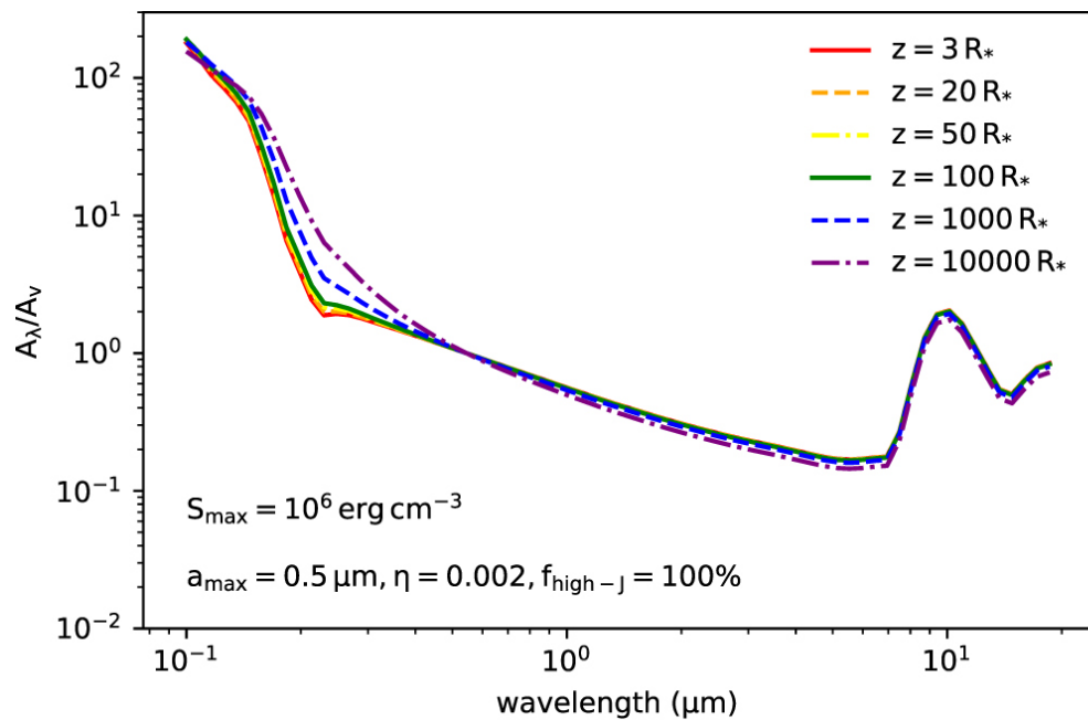
Figure 9. from Bao Truong et al 2022 Astrophys. J. 936 doi:10.3847/1538-4357/ac86d9 https://dx.doi.org/10.3847/1538-4357/ac86d9 © 2022. The Author(s). Published by the American Astronomical Society.
