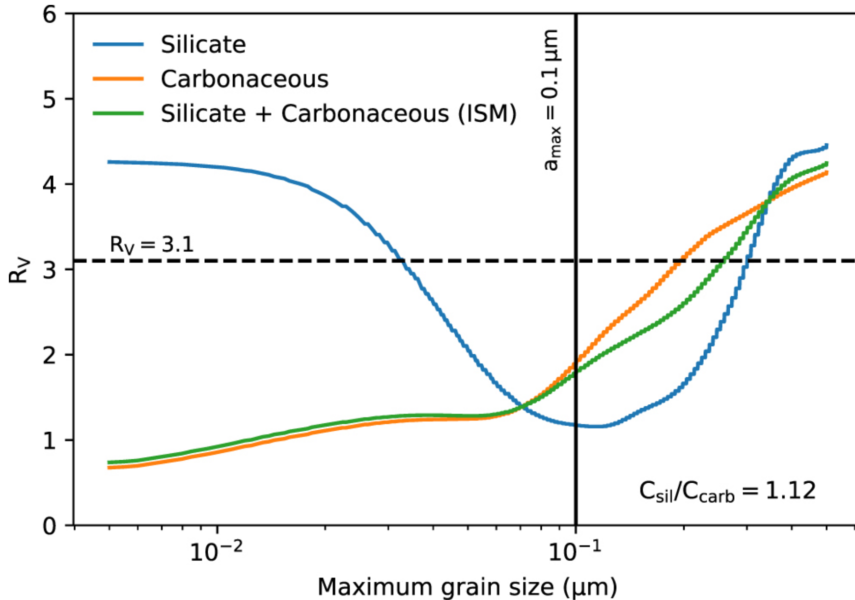
Figure 3. from Bao Truong et al 2022 Astrophys. J. 936 doi:10.3847/1538-4357/ac86d9 https://dx.doi.org/10.3847/1538-4357/ac86d9 © 2022. The Author(s). Published by the American Astronomical Society.
