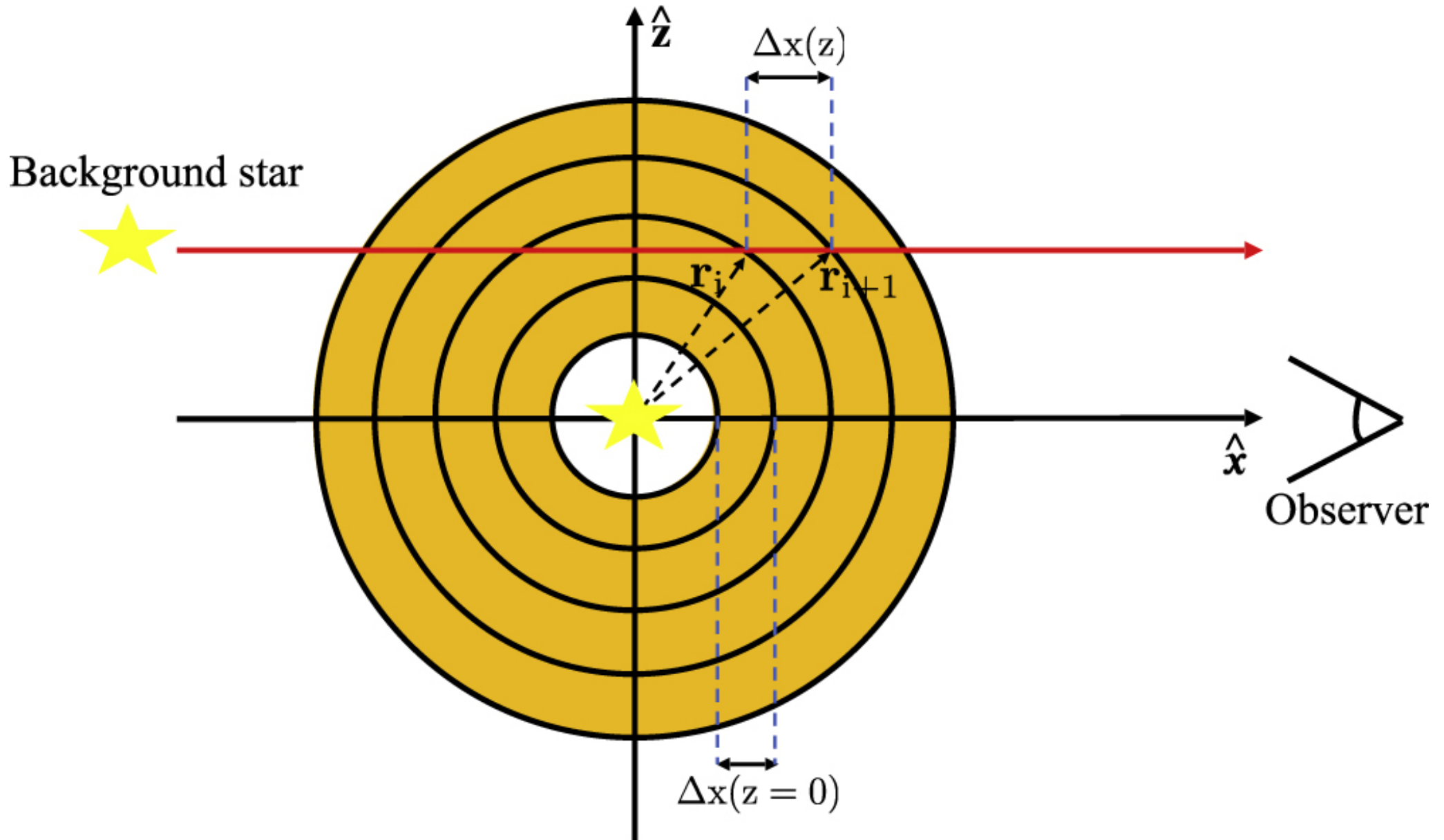
Figure 2. from Bao Truong et al 2022 Astrophys. J. 936 doi:10.3847/1538-4357/ac86d9 https://dx.doi.org/10.3847/1538-4357/ac86d9 © 2022. The Author(s). Published by the American Astronomical Society.
