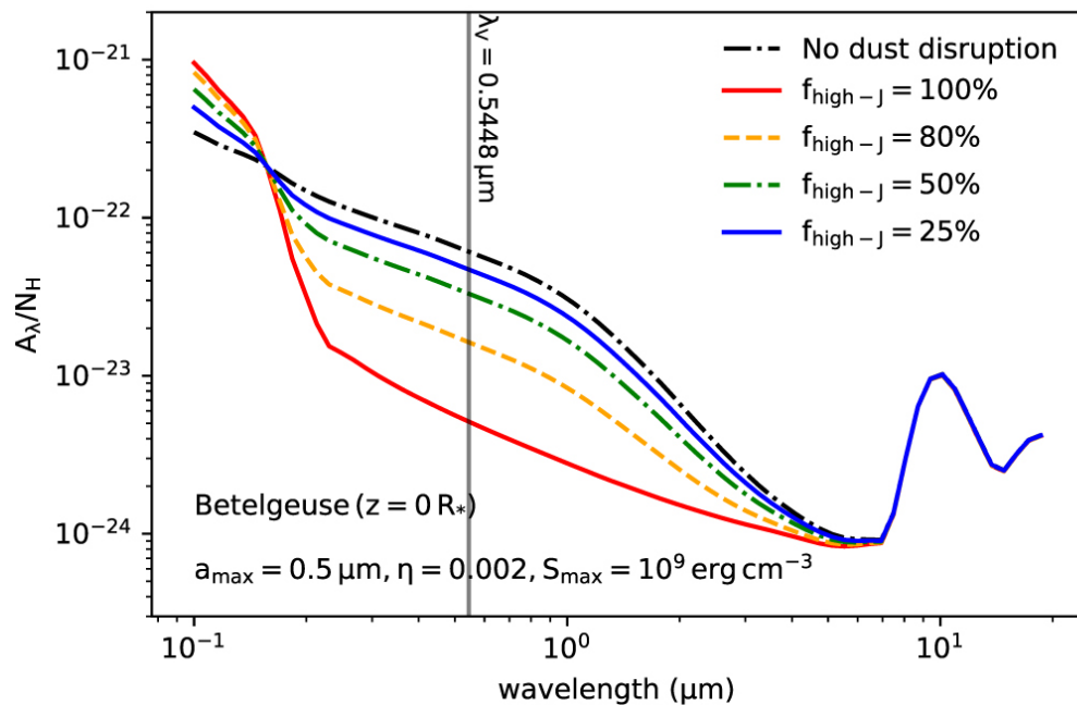
Figure 17. from Bao Truong et al 2022 Astrophys. J. 936 doi:10.3847/1538-4357/ac86d9 https://dx.doi.org/10.3847/1538-4357/ac86d9 © 2022. The Author(s). Published by the American Astronomical Society.
