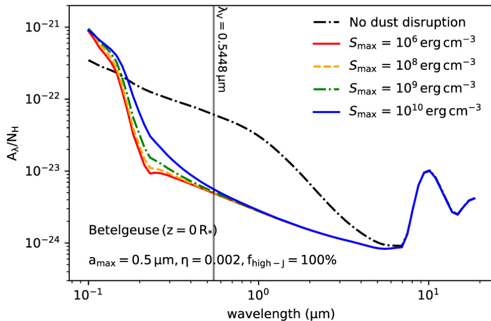
Figure 16. from Bao Truong et al 2022 Astrophys. J. 936 doi:10.3847/1538-4357/ac86d9 https://dx.doi.org/10.3847/1538-4357/ac86d9 © 2022. The Author(s). Published by the American Astronomical Society.
