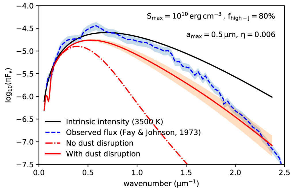
Figure 15. from Bao Truong et al 2022 Astrophys. J. 936 doi:10.3847/1538-4357/ac86d9 https://dx.doi.org/10.3847/1538-4357/ac86d9 © 2022. The Author(s). Published by the American Astronomical Society.
